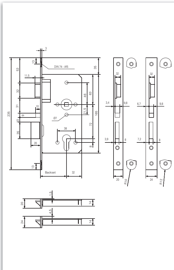
Dimensioning: GBS 91
